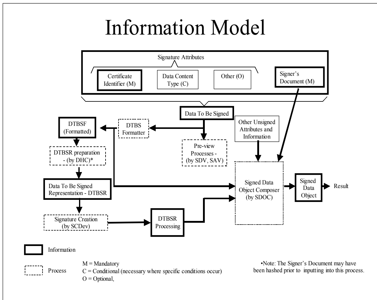
Figure 4 – Information Model of Advanced or, where applicable, Qualified Electronic Signature creation
