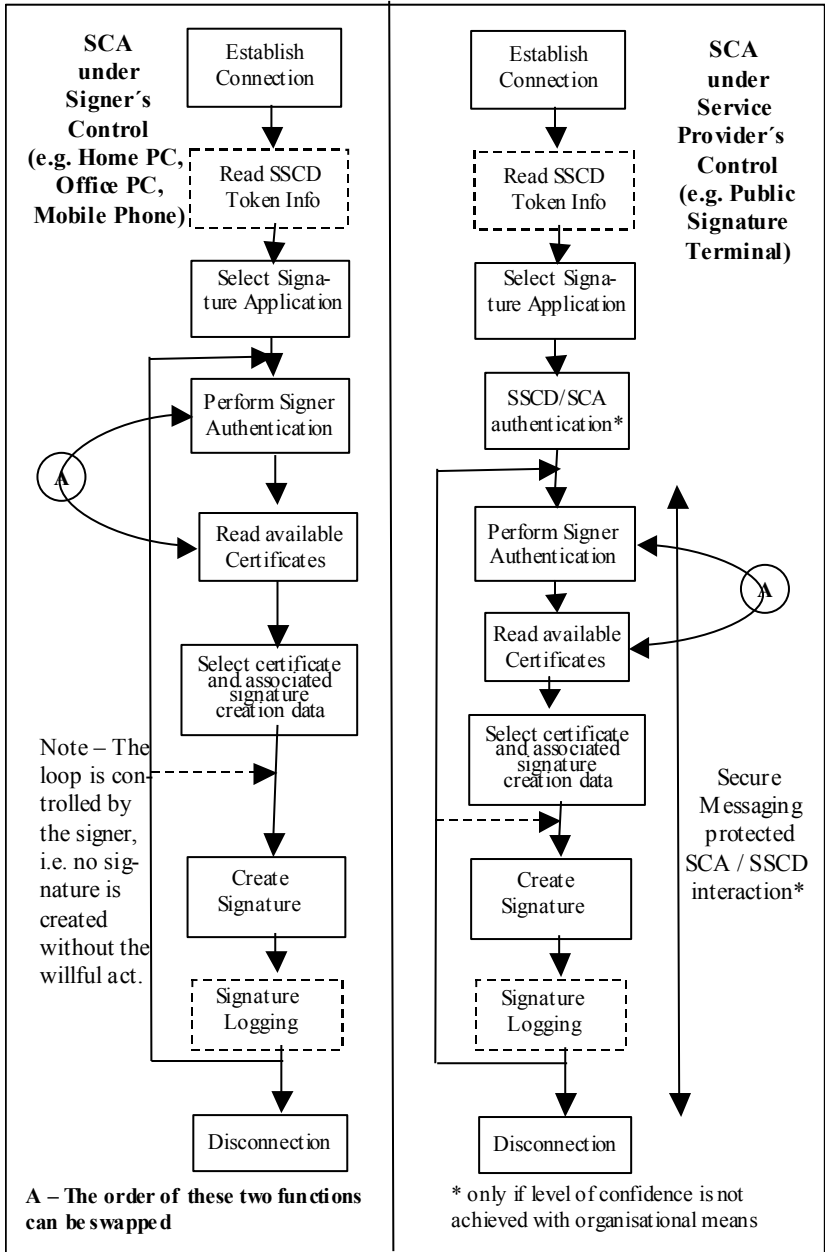
Figure 8 - Interaction sequences between SCA and SCDev
