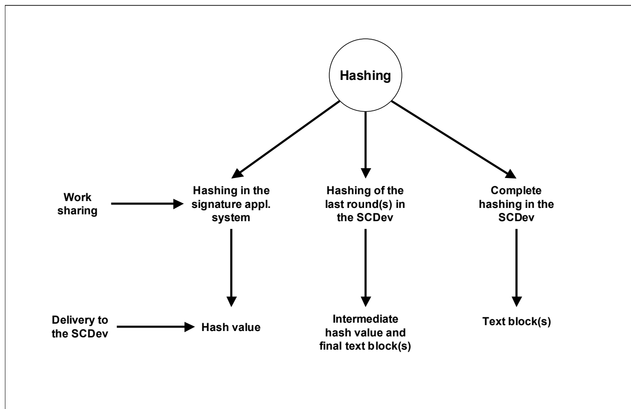
Figure 7 - Possible work sharing for hashing
