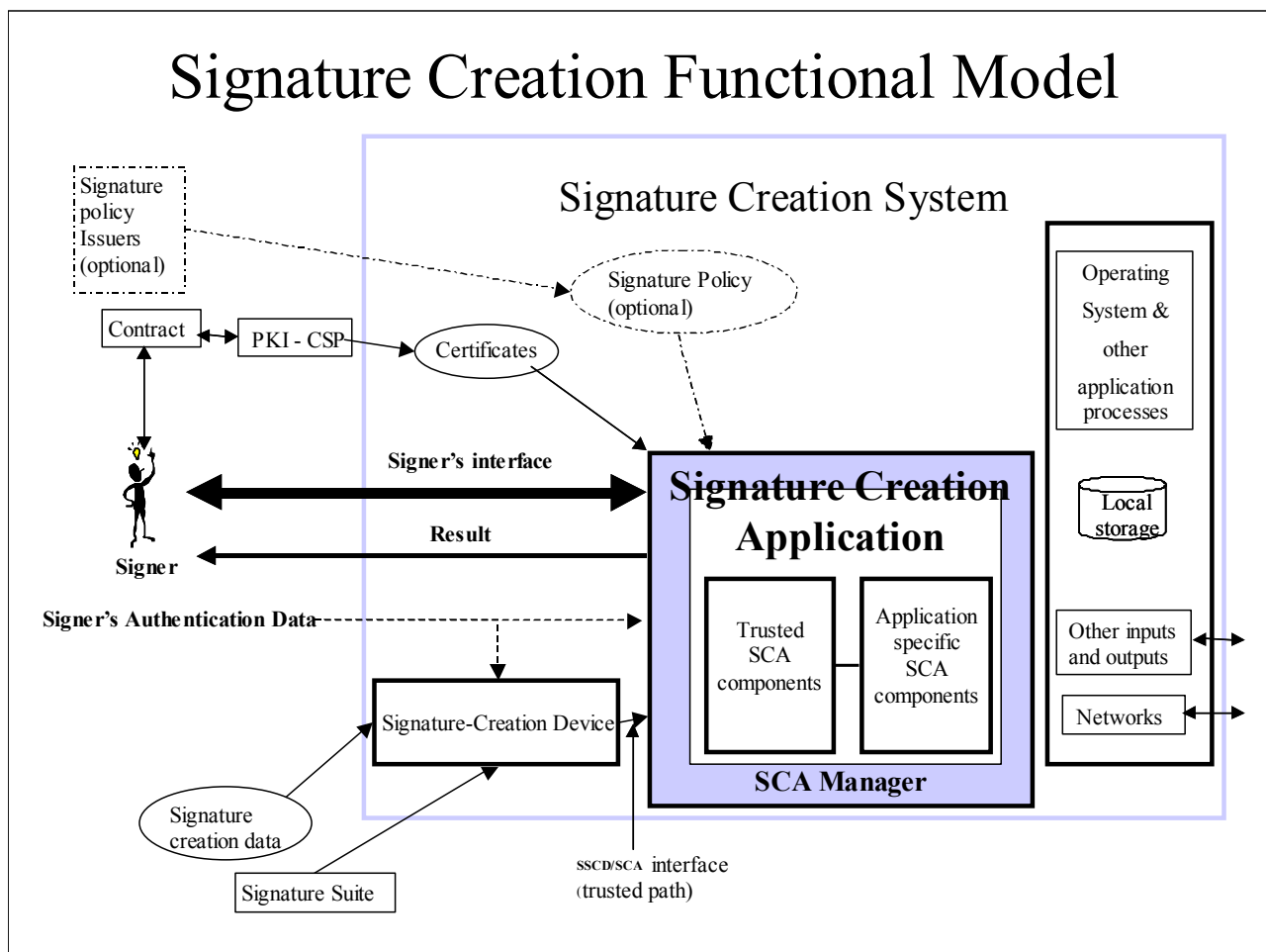
Figure 1 – The Signature Creation Functional Model
