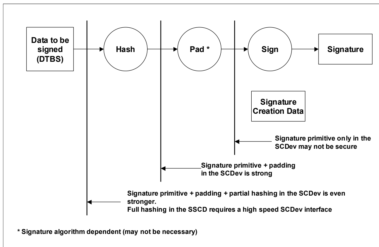
Figure 6 - Signature process and possible work sharing between SCA and SCDev
