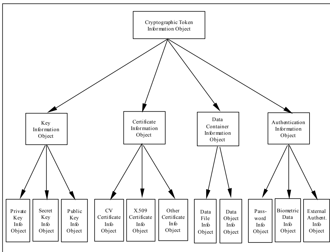
Figure 9 – Example: SCDev data elements to be described by the cryptographic token information objects
