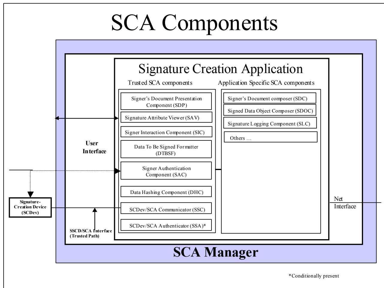
Figure 2 - SCA Components
