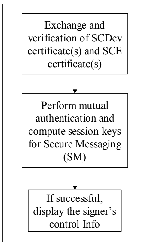
Figure 10 - Steps of authentication process between SCA and SCDev
